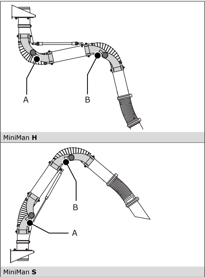
Fig. 6.1 Adjustment points
