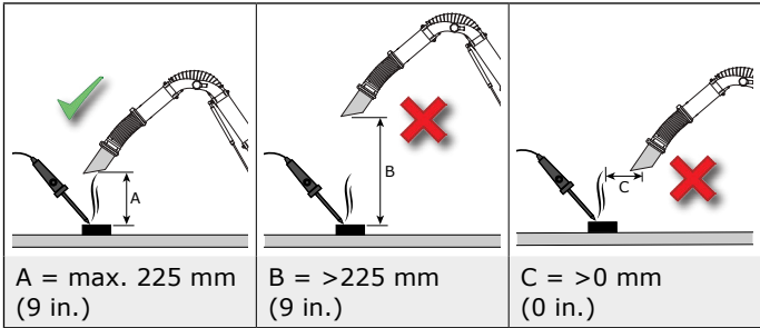
Fig. 5.1 A = Correct position of the nozzle (example: soldering)
