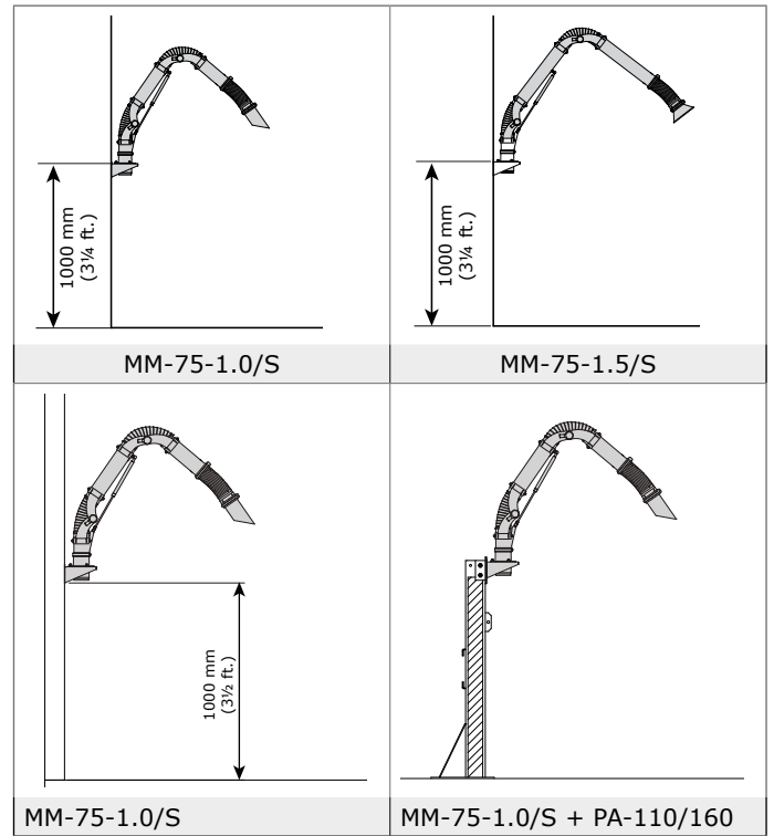
Fig. IV Mounting examples MiniMan S
