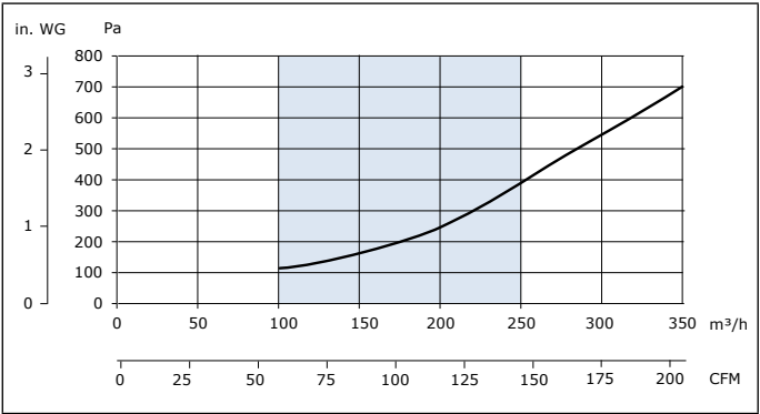
Fig. II Pressure drop
