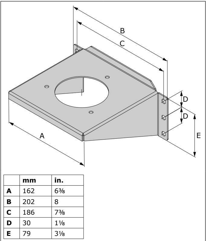
Fig. 4.2 Mounting bracket
